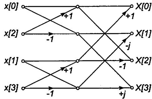
Figure 8.4: Butterfly diagram of a decimation-in-time radix-2 FFT for N = 4 . Any branches not marked have a gain of +1 .
