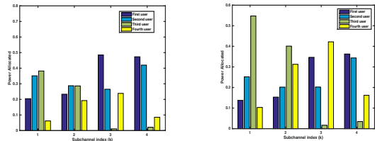
(a) Total Power Constraint. (b) Per Transmitter Constraint.
